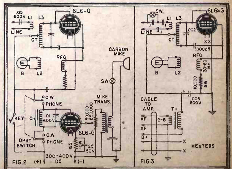
Fig. 2—The 6L6 modulator and transmitter circuit complete. Fig. 3—A suitable hook-up for use if an audio amplifier is available as modulator. Values for all coils are supplied in the text.
