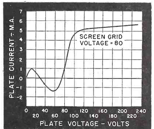
Fig. 3—"Dynatron kink" of a tetrode tube.
