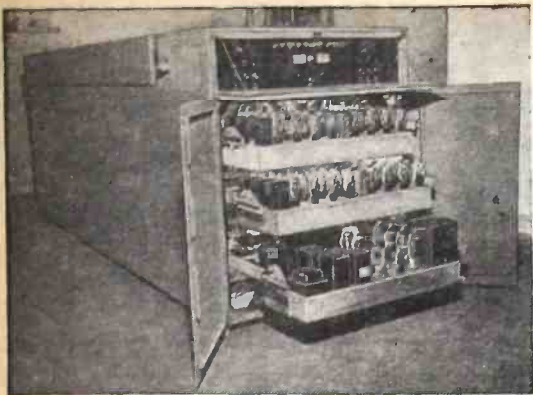
Ground-base receiving and recording unit of electronic flight recorder. Count the tubes.
