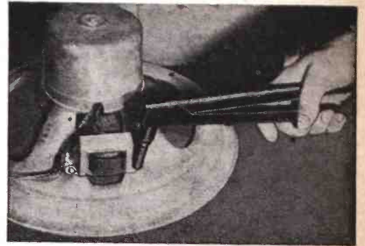
Fastening an output transformer to speaker.
