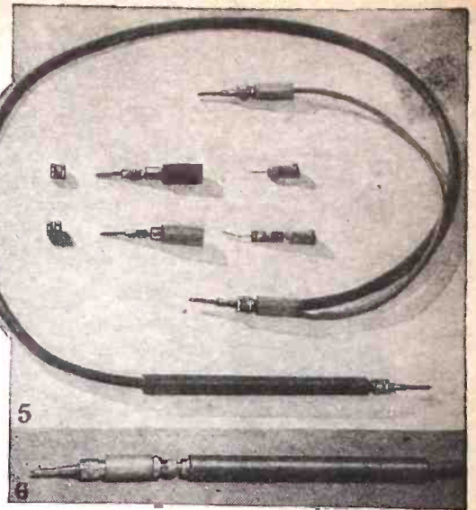
Photo 4, above—Under-chassis view of tracer. 5 and 6 Construction of the signal prods.
