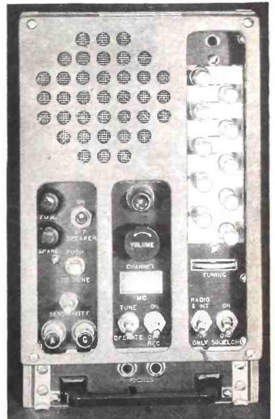
Fig. 2—The BC-603 receiver. Lamp above volume control lights when signals are received.
