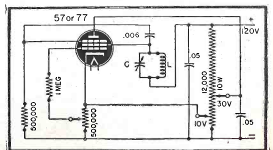
Fig. 4—Circuit of a Transitron oscillator.
