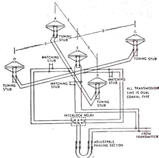
Method of feeding 5-loop radio range antenna.
